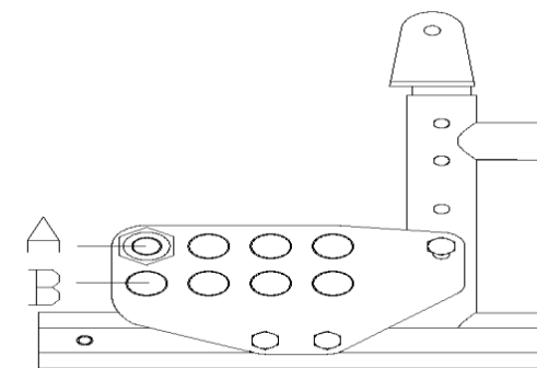
20", 22" WHEEL AXLE PLATE
